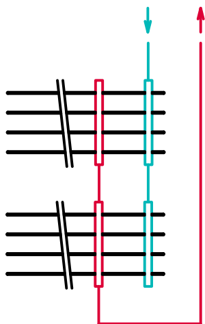
Alternate method for connecting two Energy Blades
