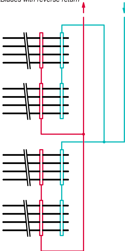
Connecting four or more Energy Blades with reverse return
